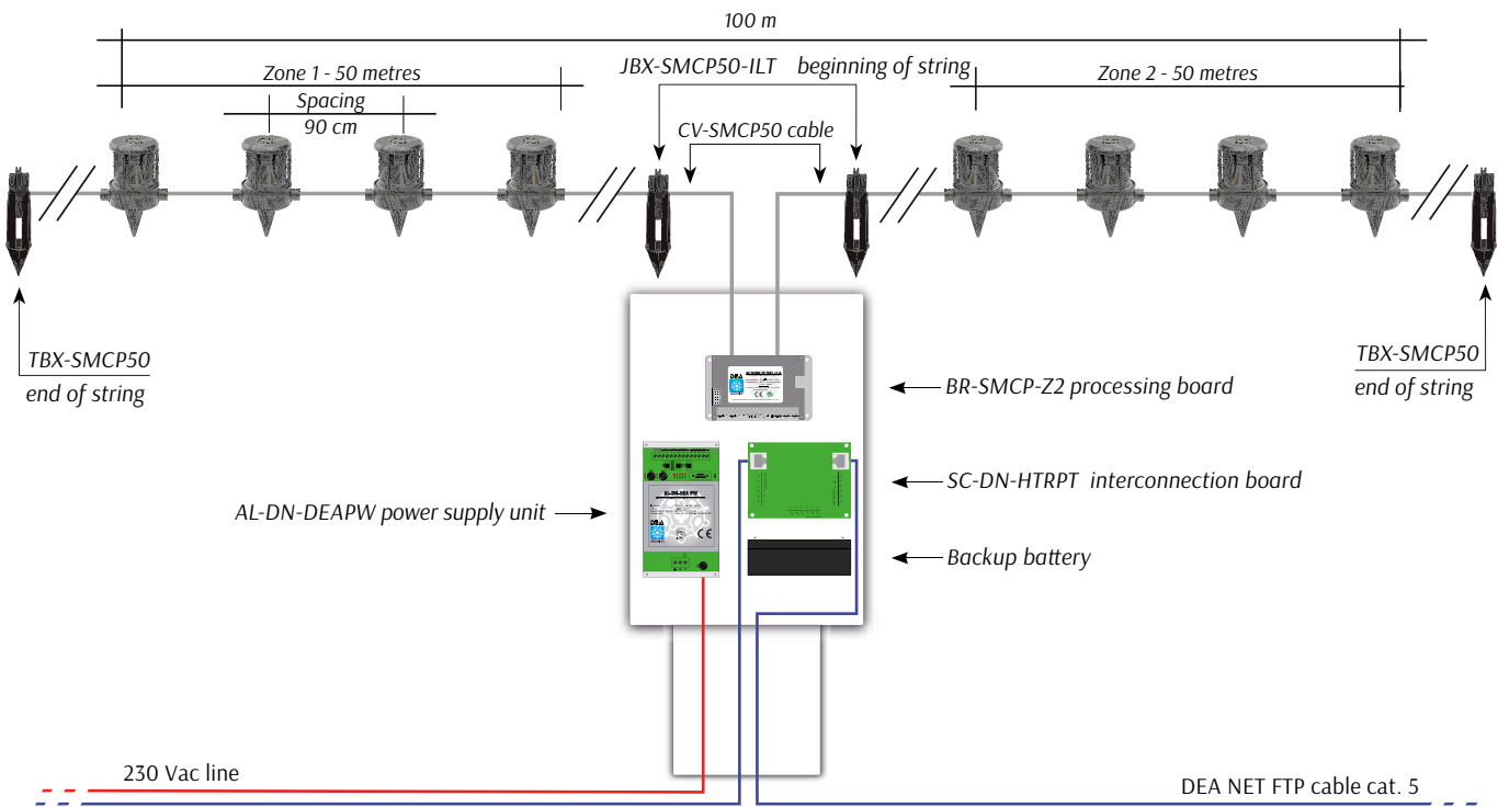
TYPICAL CONFIGURATION OF A SISMA CP 50 FIELD CABINET (2 ZONES)
